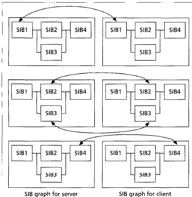
■ Figure 7. The active SIBs in the SIB graphs directly communicate with the corresponding ones at each time instant.
